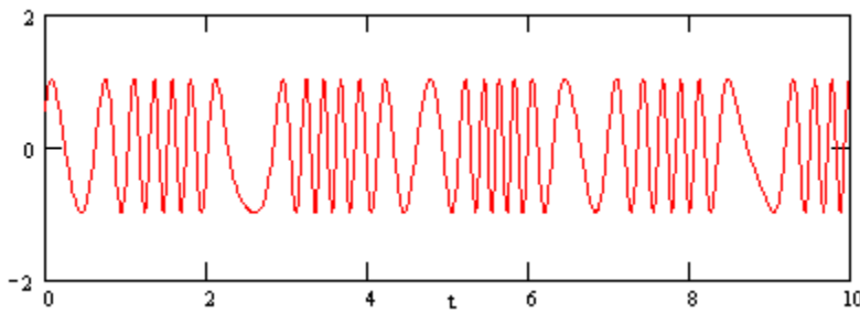
b. Phase modulation is response to an analog message. The phase changes are smooth.
