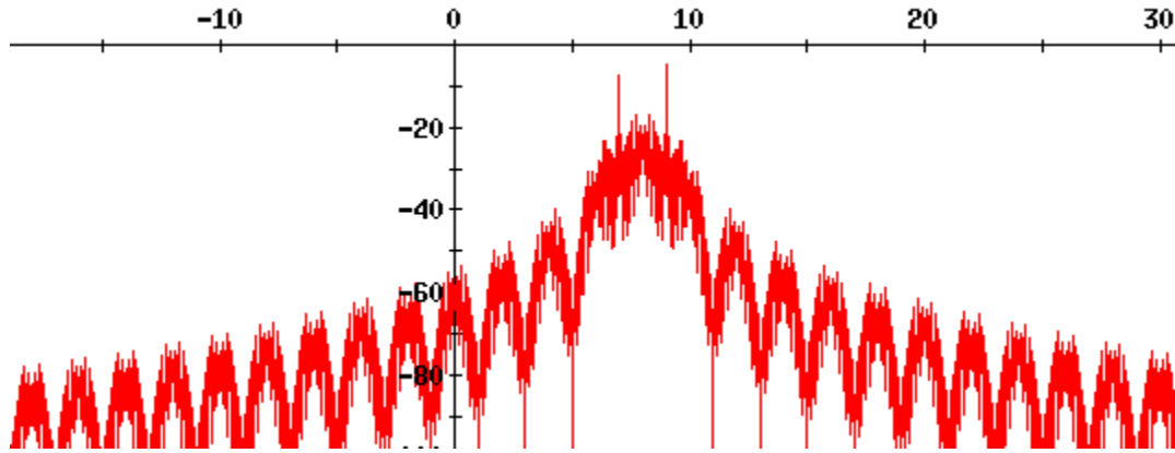
Figure 11 – Sunde’s FSK spectrum with tones at = 9 and 7 Hz.
