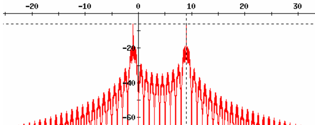
c. Spectrum shows two impulses at f ; 5 + 4 = 9 and 4 - 5 = -1
