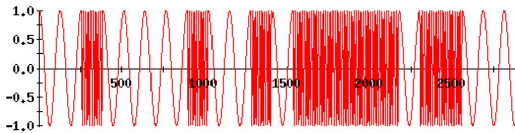
b. Modulated signal f_c = 4 , D\delta f = 5
