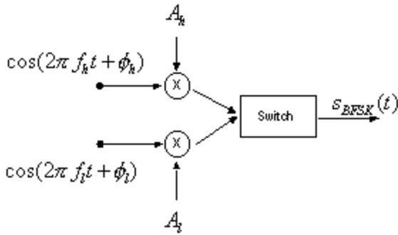
Figure 7 – A FSK modulator
