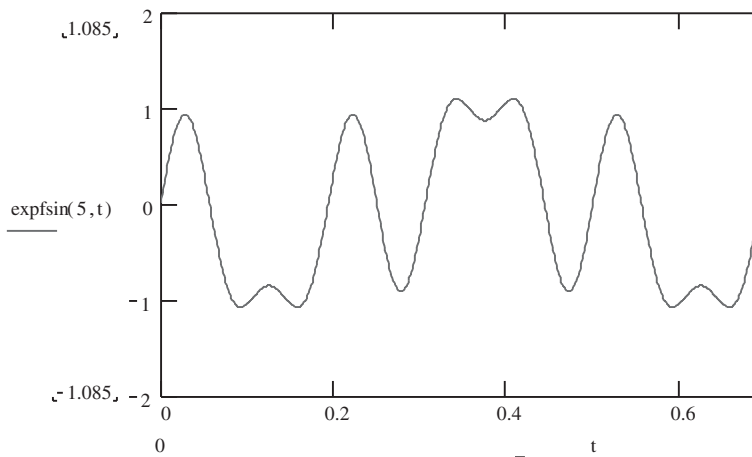
Figure 16 – Plot of \sin(k_f \sin \omega_m t) = \underline{2J_1(k_f)} \sin(\omega_m t) + \underline{2J_3(k_f)} \sin(3\omega_m t) + \underline{2J_5(k_f)} \sin(5\omega_m t) + \dots
