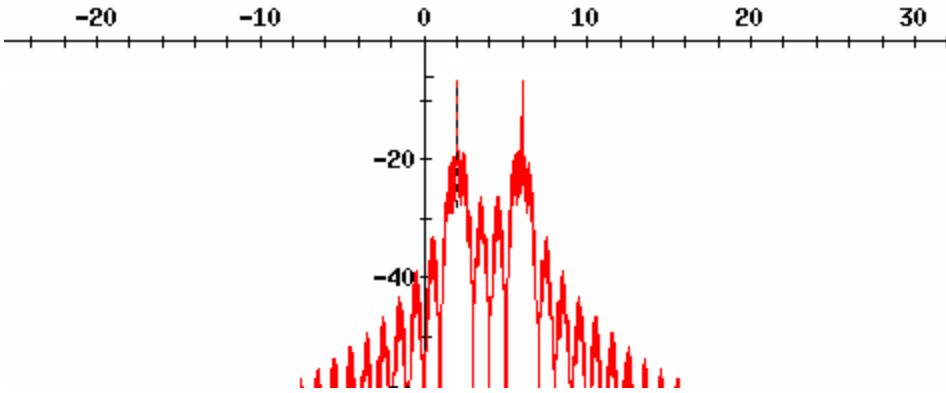
Figure 9- Spectrum of the modulated signal, D\delta f is equal 2. Note the two impulses at frequencies 2 and 6 Hz.
