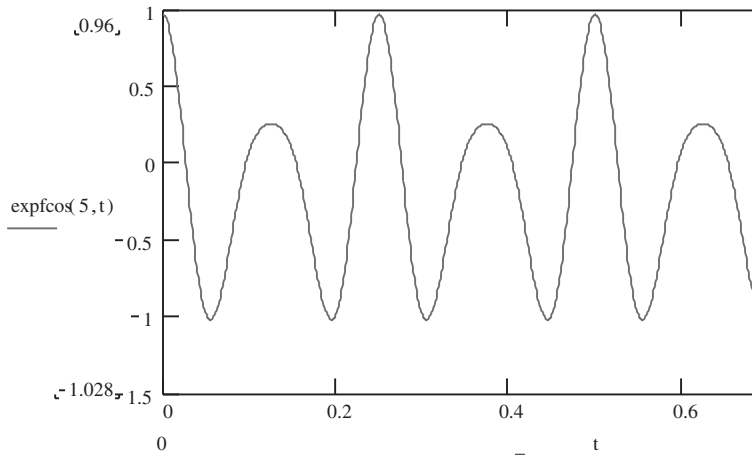
Figure 15 – Plot of \cos(k_f \sin \omega_m t) = \underline{J_0(k_f)} + \underline{2J_2(k_f)} \cos(2\omega_m t) + \underline{2J_4(k_f)} \cos(4\omega_m t) + \dots
