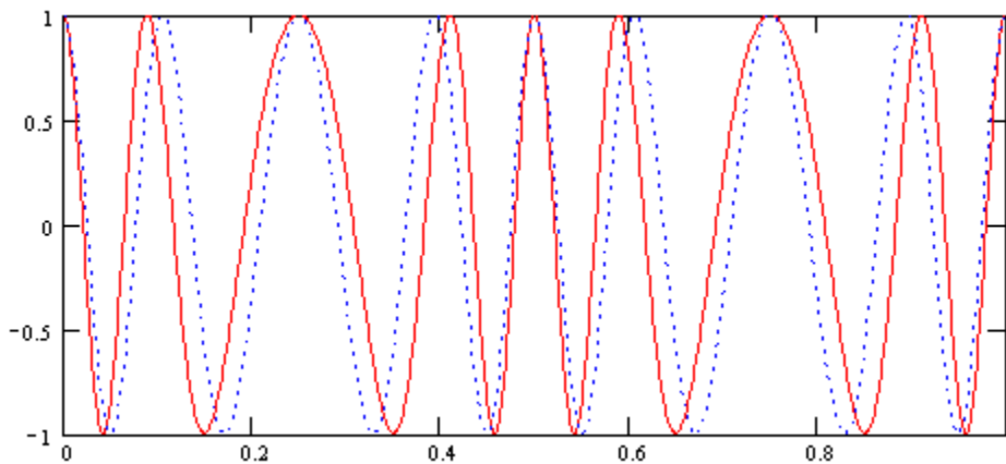
Figure 17 – Modulated FM signal for k_f = 2 and k_f = 1 , the red signal is moving faster indicated higher frequency components .
