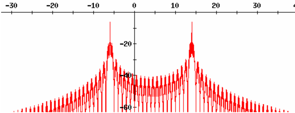
e. Spectrum shows two impulses at f ; 10 + 4 = 14 and 4 - 10 = -6 Note that the spectrum does look like a superposition of impulses and sinc functions.
