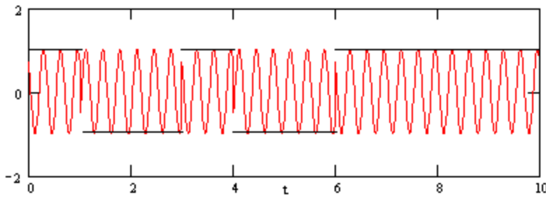
a. Phase modulation is response to a binary message. The phase changes are abrupt.
